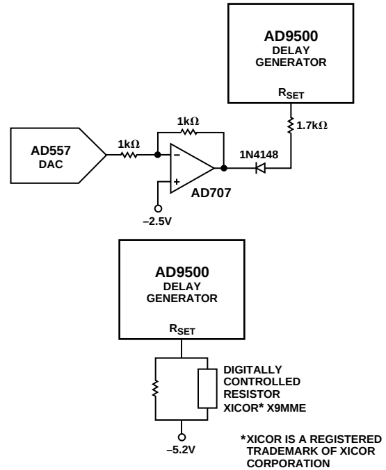
Figure 5. Programmable Full-Scale Range Using a DAC or a Digitally Controlled Resistor
