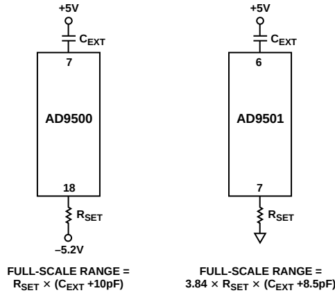
Figure 3. Setting Full-Scale Range on the AD9500 and AD9501
