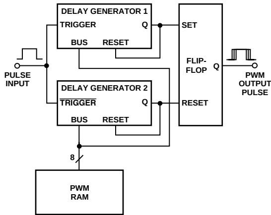
Figure 12. Laser Printer PWM
