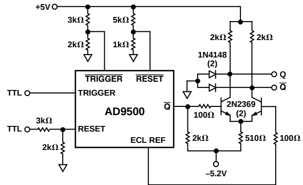
Figure 7. Interfacing the AD9500 with TTL
