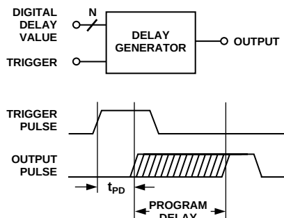
Figure 1. Programmable Delay Generator
