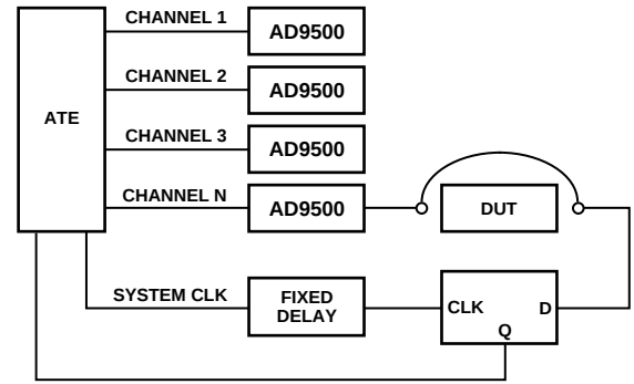
Figure 11. Automatic Calibration for ATE Deskew
