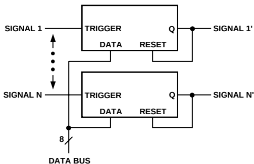
Figure 10. Multiple Signal Deskewing
