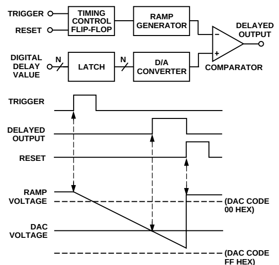
Figure 2. Delay Generator Block Diagram and Basic Timing
