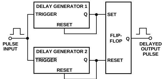
Figure 9. Two Delay Generators Used to Delay Both Input Pulse Edges to Main Pulsewidth at the Output
