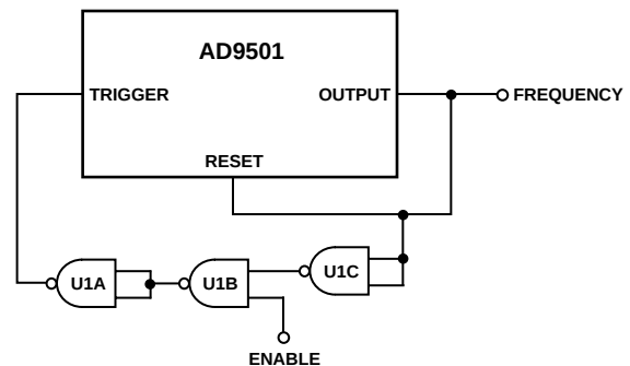
Figure 8. The AD9501 Configured as a Programmable Oscillator
