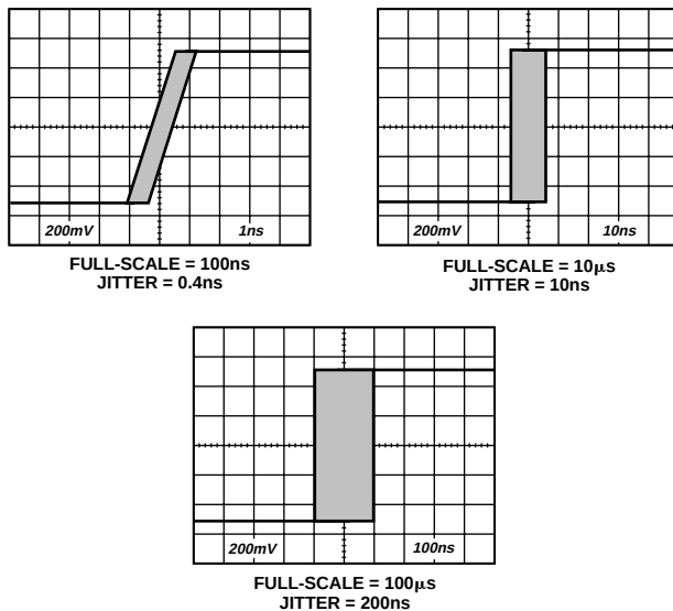
Figure 4. Output Jitter at Various Full-Scale Settings for the AD9500 and AD9501
